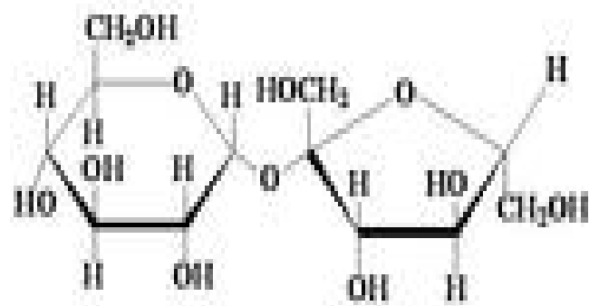
sucrose
