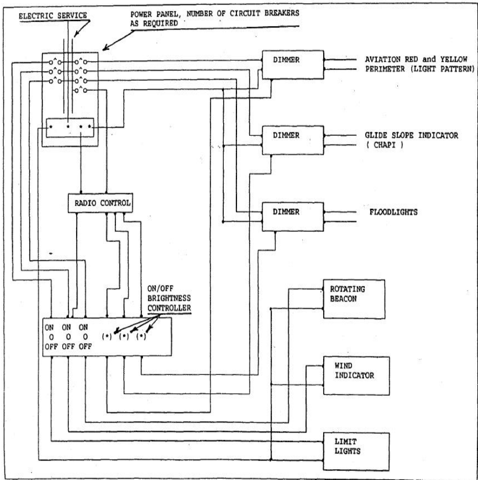
FIGURE 11-3. HOSPITAL HELIPAD LIGHTING CONTROL DIAGRAM
