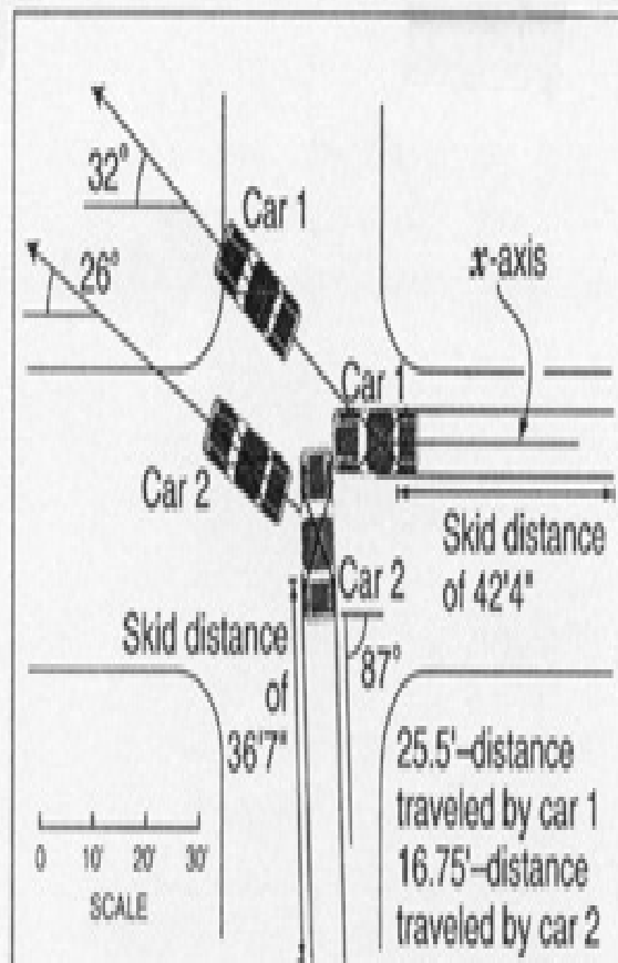
Fig. 2. Scale drawing showing the position of the cars at impact and the final resting positions after the accident
