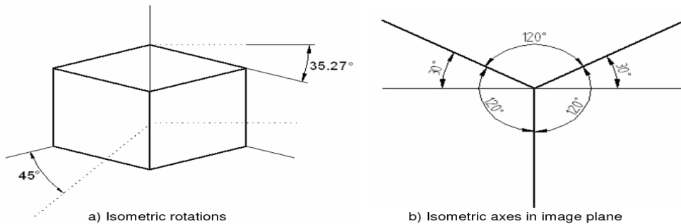
Fig. 1 Isometric projection
