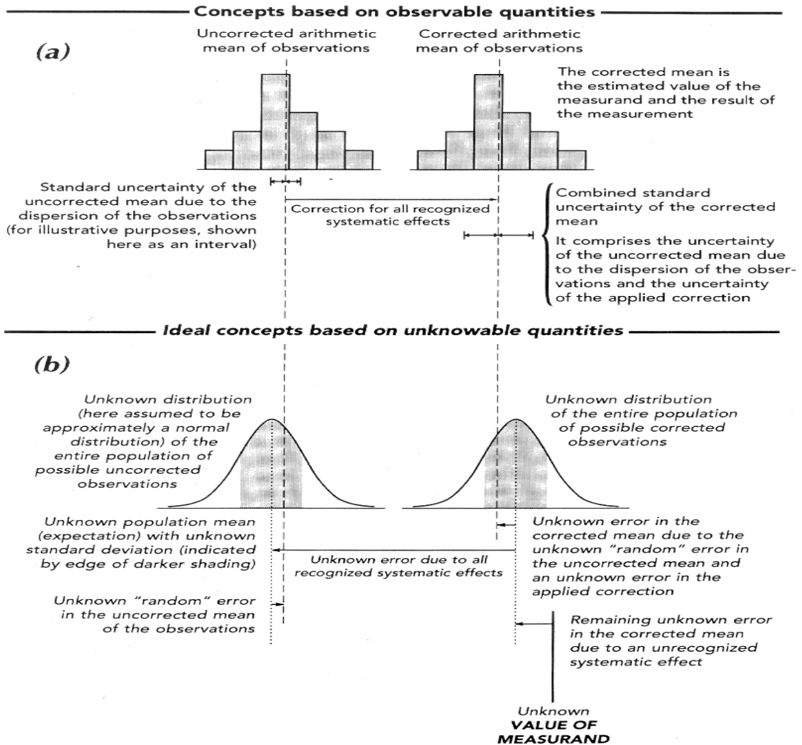
Figure D.1. Graphical illustration of value, error, and uncertainty
