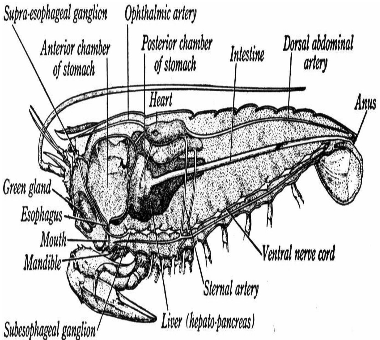
FIG. 248. Internal Anatomy of the Crayfish 1
