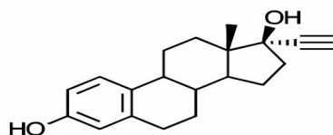
Mestranol (Norgestrel)
