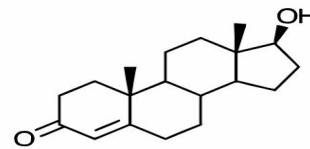
Testosterone
