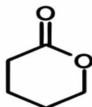
Lactone
