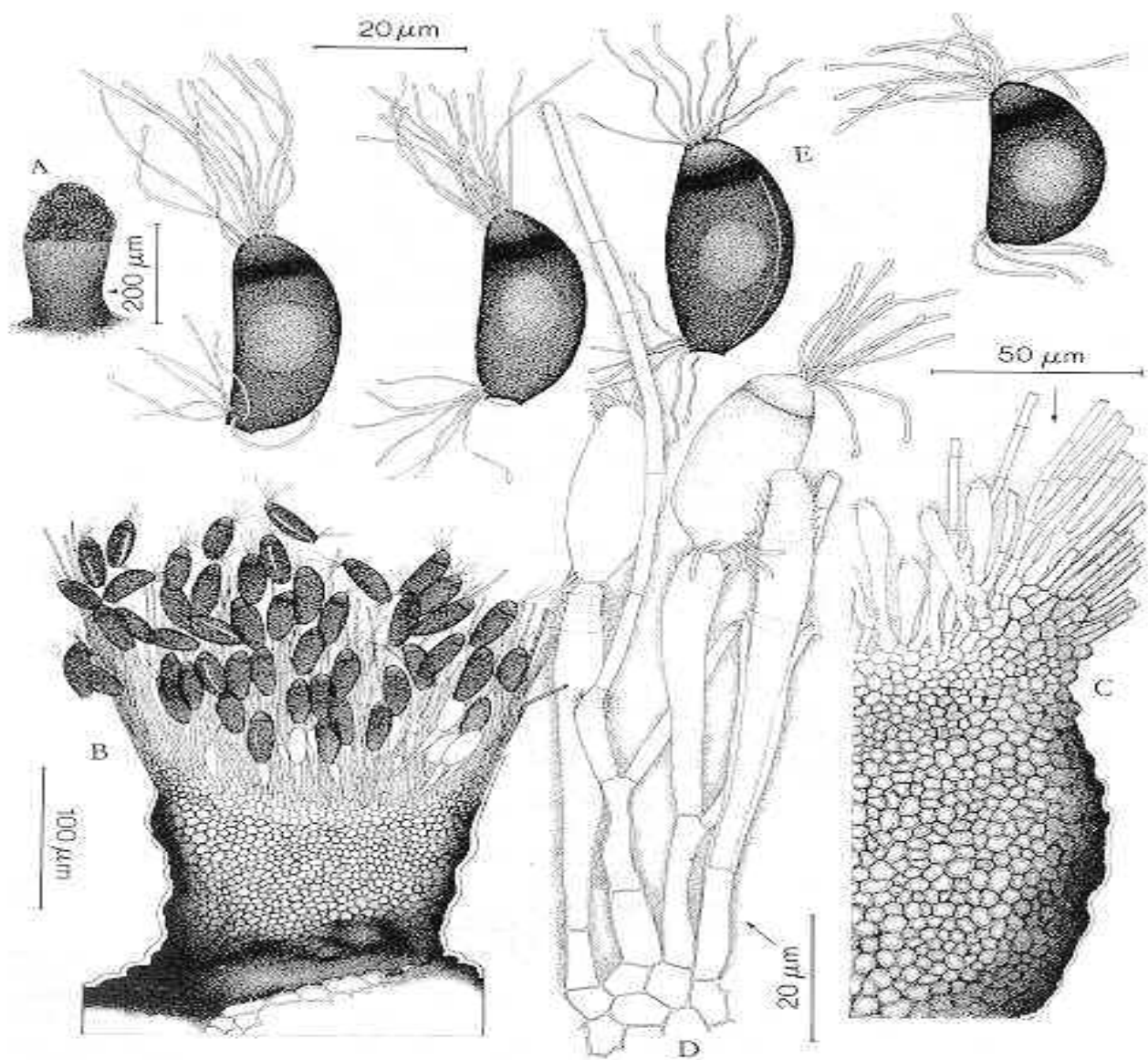
Figure 120.1. Stevensonula ciliata ex holotype in W. A. Habit sketch of a conidioma. B. Vertical section of a conidioma. C. Enlarged partial view of a conidioma showing tissue details. D. Conidiogenous cells with developing conidia. E. Mature conidia.
