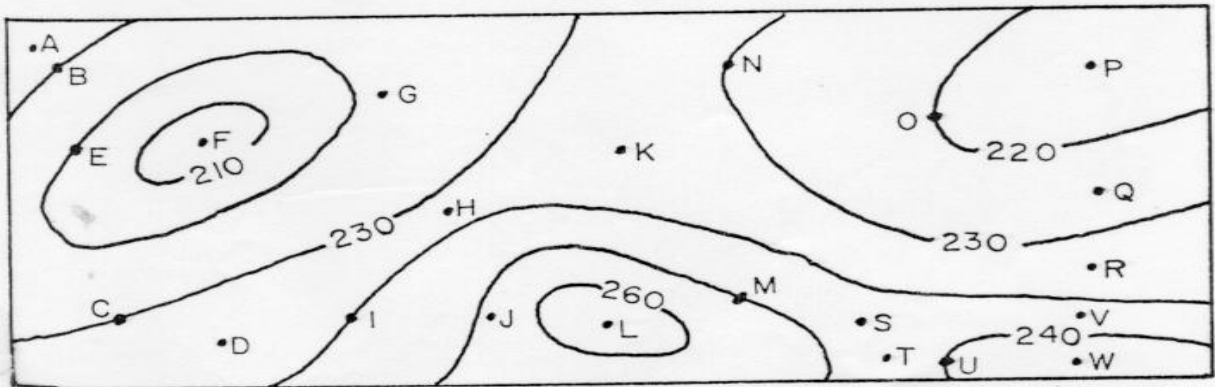
MAP C ISOPLETH INTERVAL = 10
