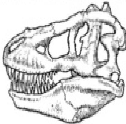
Tyrannosaurus rex
