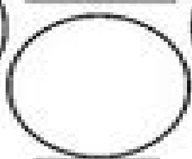
Full Moon
