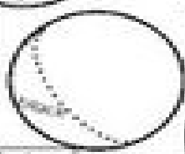
Waxing Gibbous
