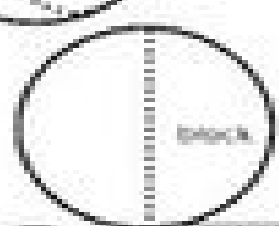
Waning Quarter
