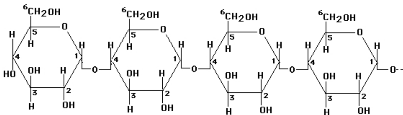
(a) Amylose (Glucose- \alpha (1-4)-Glucose)
