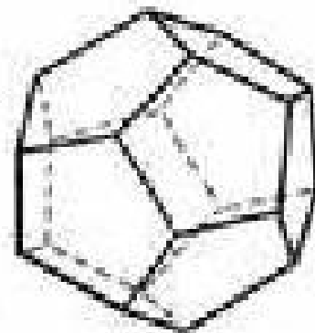
Dodecahedron
