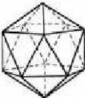
Icosahedron
