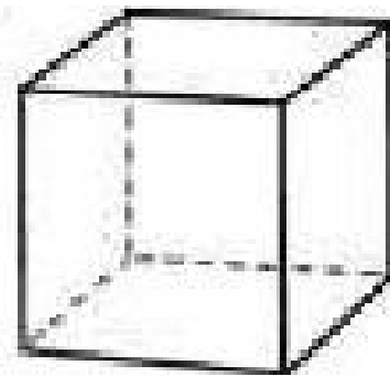
Cube
