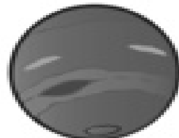
Neptune
