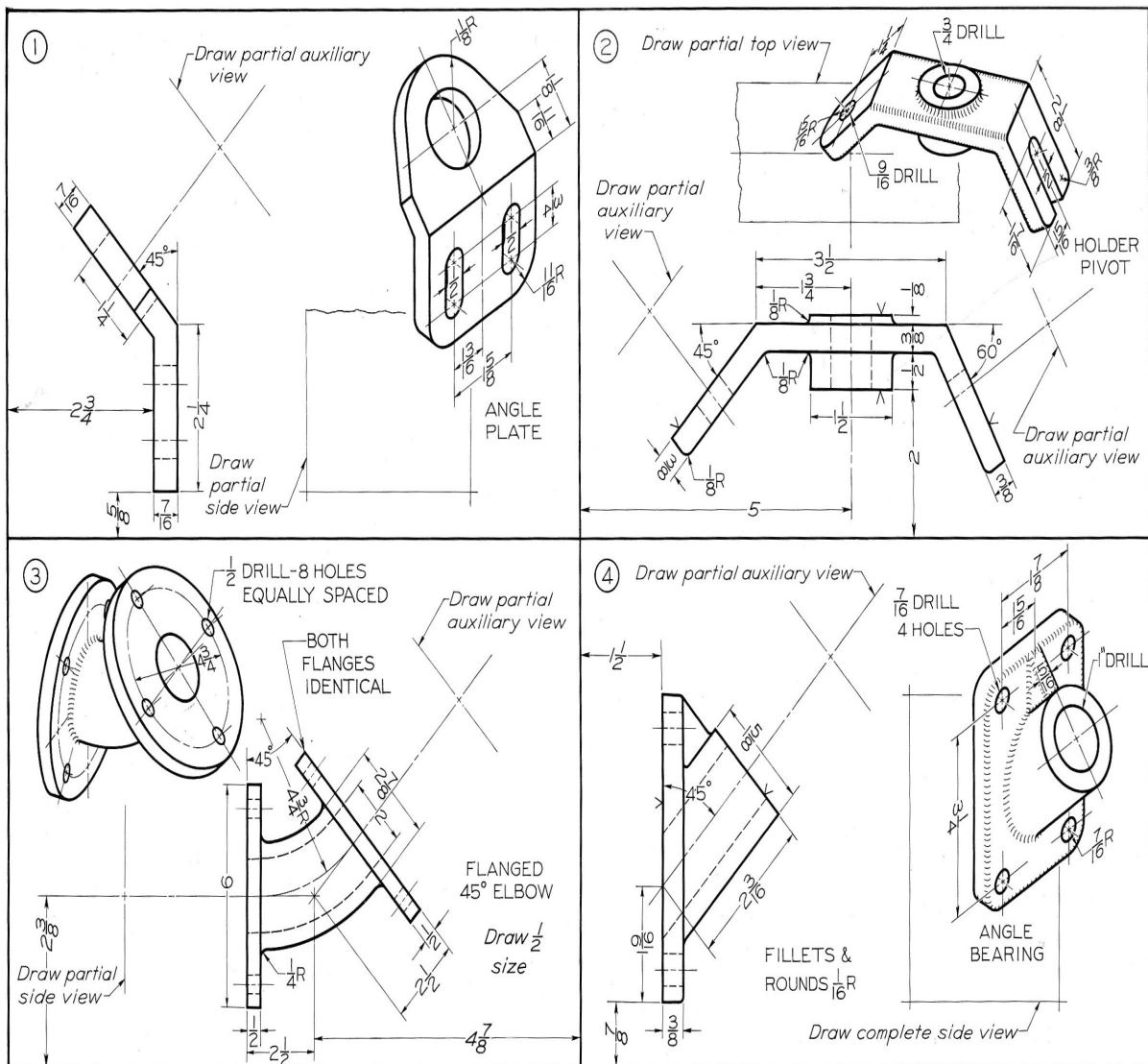
Fig. 12-20. Auxiliary-View Problems. Using Layout C (Appendix, page 474), make complete mechanical drawing of problem assigned. Omit pictorial drawings, spacing dimensions, and instructional notes. Include complete dimensions, moving dimensions from pictorials to the views.
