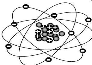
Atom B
