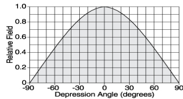
E-plane Vertical pattern – V-polarization
