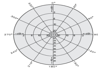
H-plane Horizontal pattern – V-polarization
