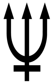
Neptune
