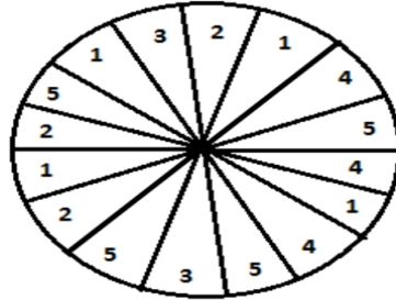
Probability - Spinner
