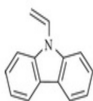
NVC
