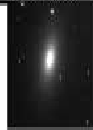
M59 Elliptical, E5
