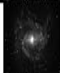
M83 Spiral, Sc
