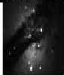
Centaurus A Peculiar, P
