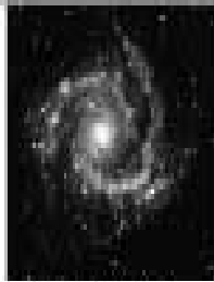
NGC 2997 Spiral, Sb
