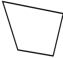
Convex
