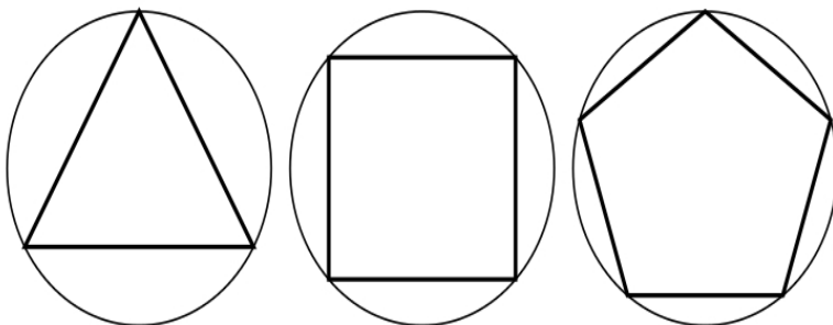
Regular convex
