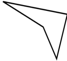
Concave
