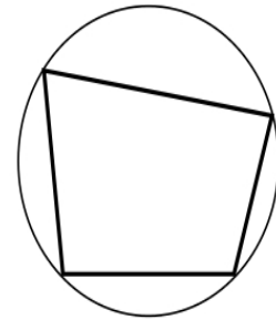
Cyclic
