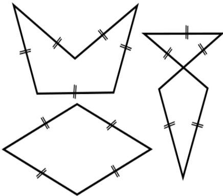
Equilateral
