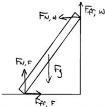
ladder leaning against wall – both wall and floor have friction
