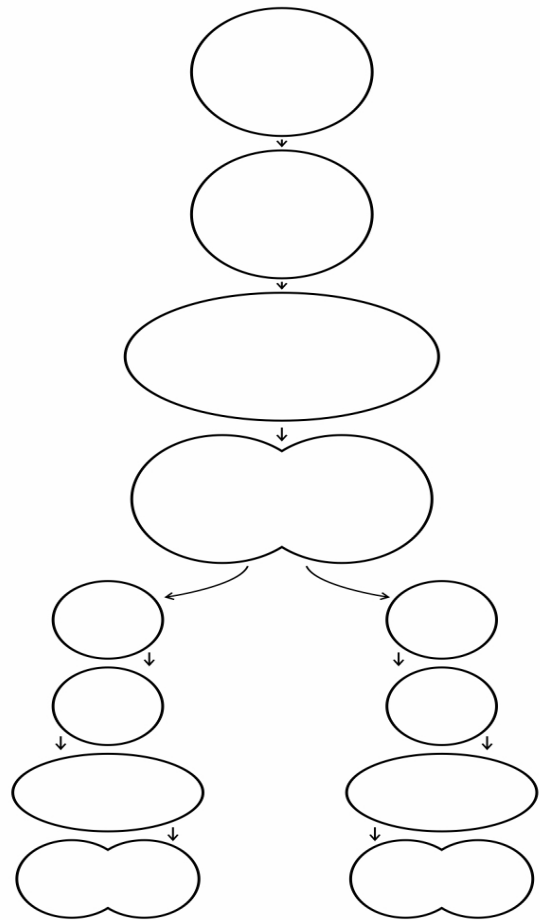
Meiosis
