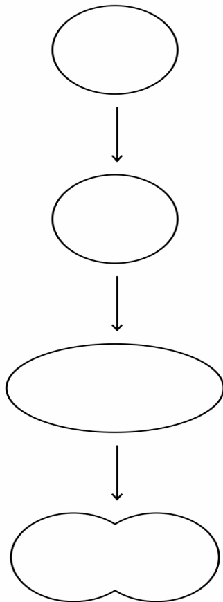
Mitosis
