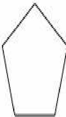
Regular Pentagon
