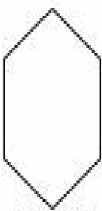
Regular Hexagon
