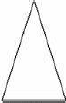
Equilateral Triangle
