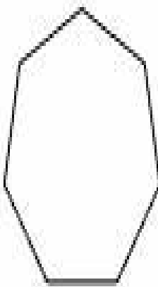
Regular Heptagon
