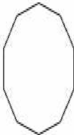
Regular Decagon
