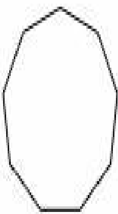
Regular Nonagon
