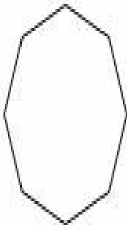
Regular Octagon
