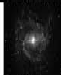
M83 Spiral, Sc
