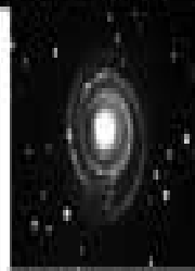
NGC 4622 Spiral, Sb
