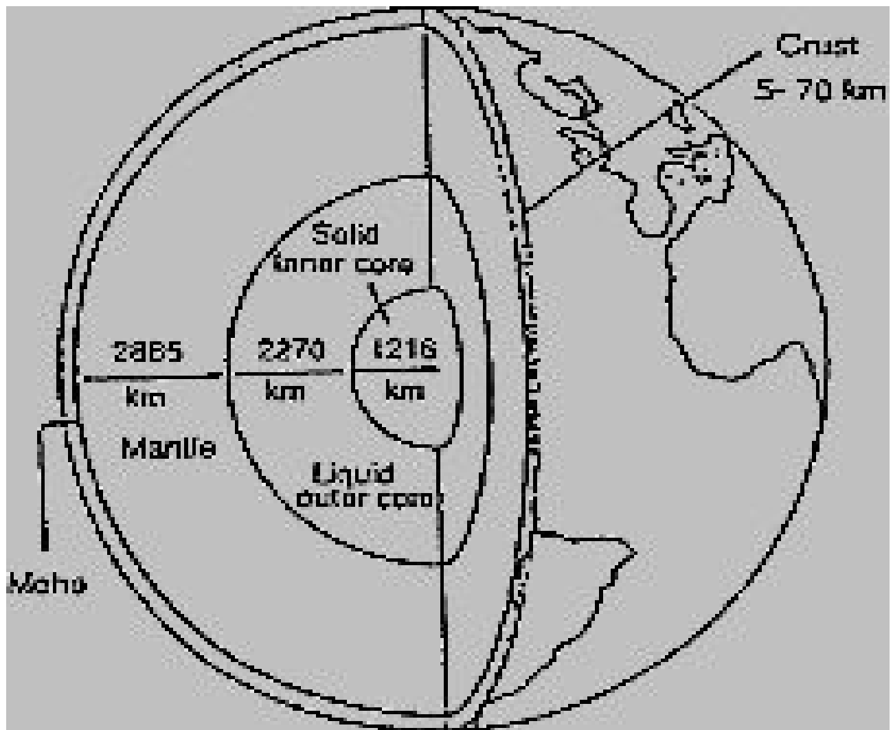
Figure 1. The Earth's layers. The Moho is the boundary between crust and mantle. Modified from NSTA/FEMA (1988).
