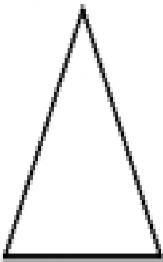
Equilateral
