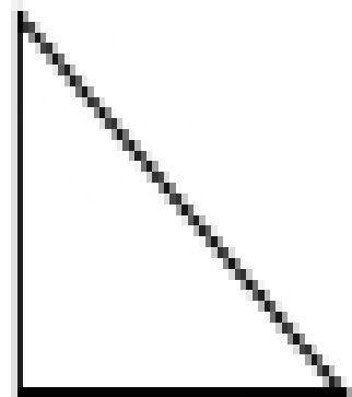
Right
