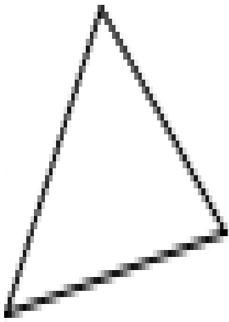
Acute
