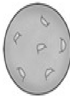
Mercury
