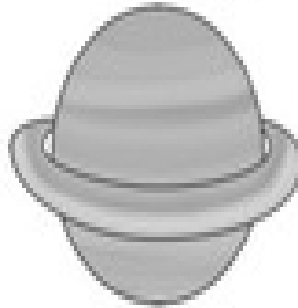
Saturn
