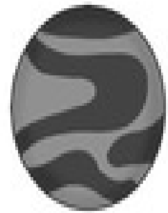
Neptune
