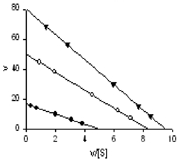
Eadie-Hofstee
