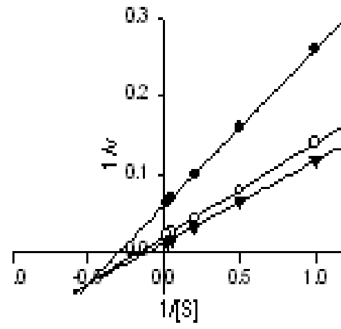
Lineweaver-Burk
