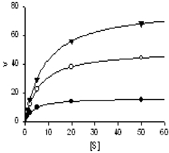
Michaelis-Menten
