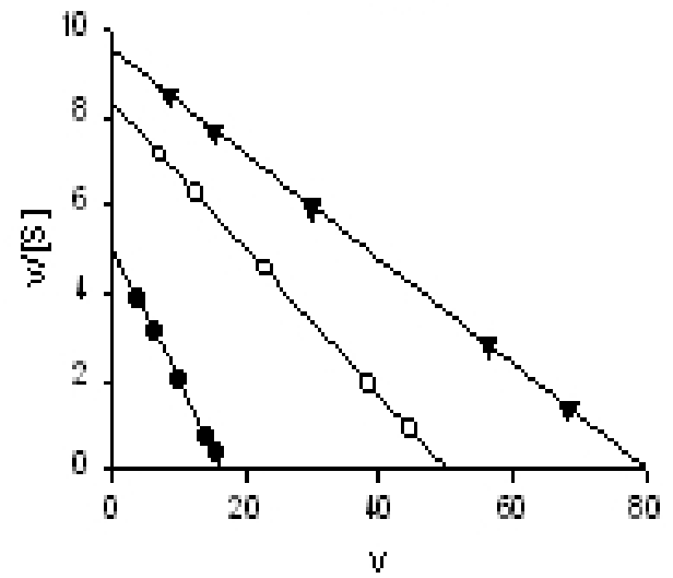
Scatchard
