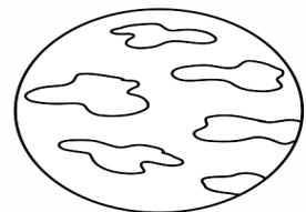
Neptune
