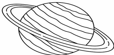
Saturn
