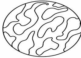
Mercury
