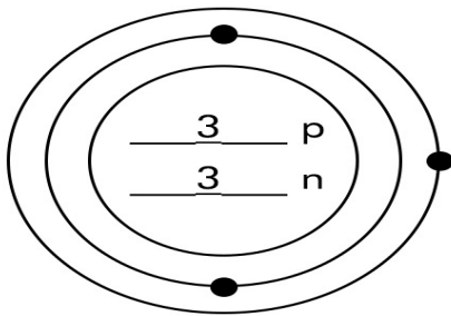
Lithium-6
