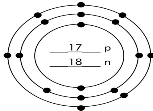
Chlorine-35
