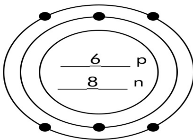
Carbon-14
