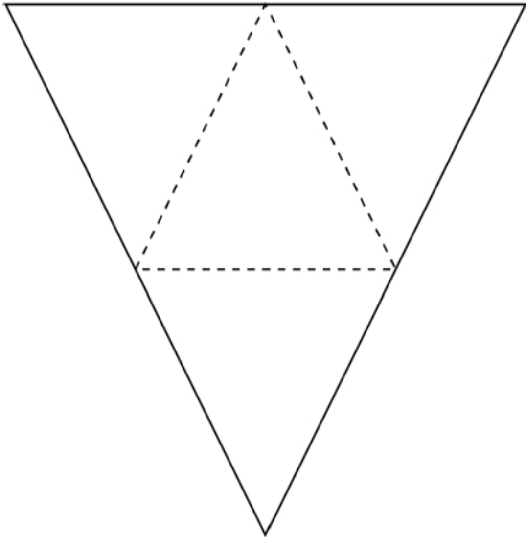
Tetrahedron
