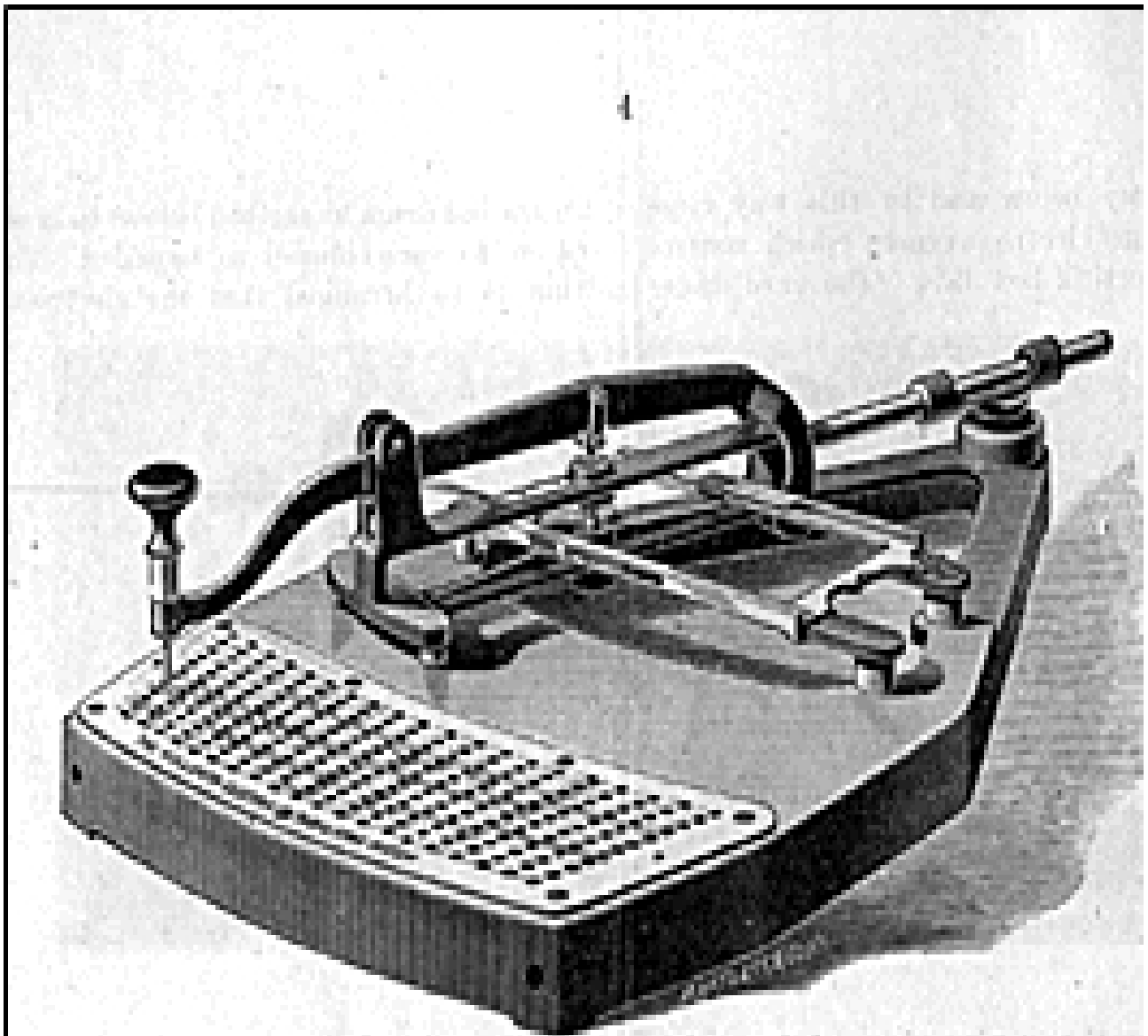
Fig. 1.—Keyboard Punch.
