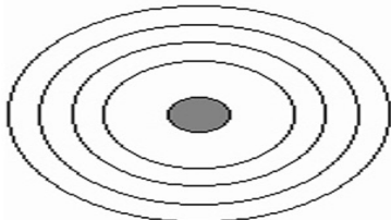
Aluminium
