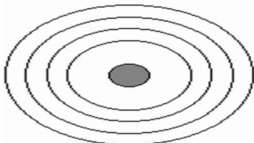
Magnesium
