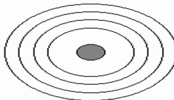
Neon
