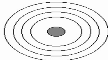
Oxygen
