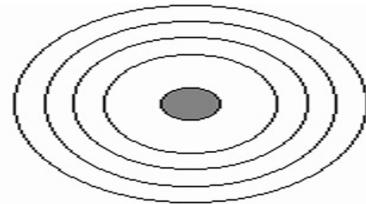
Chlorine
