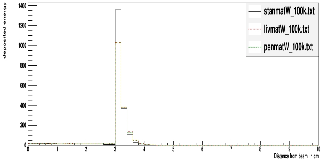
Dose, integrated over 2 bins
