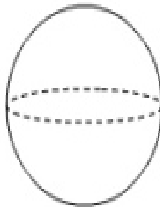
Sphere
