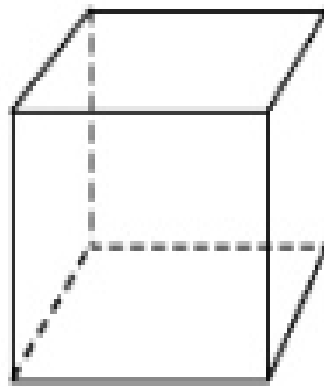
Cube
