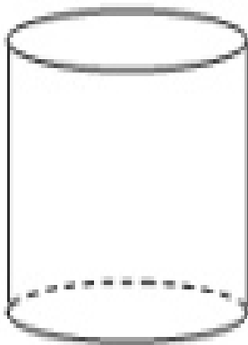
Cylinder
