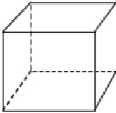
Rectangular solid
