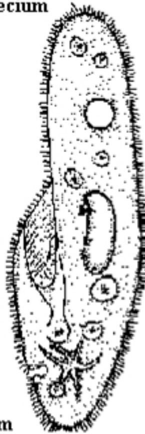
(c) Stylonychia
