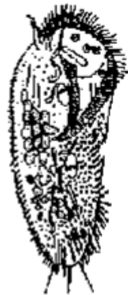
(f) Tetrahymena
