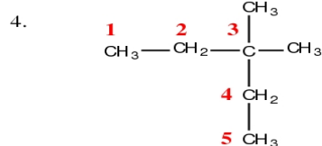
3,3-dimethylpentane
