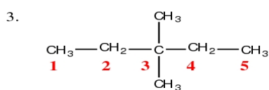
3,3-dimethylpentane
