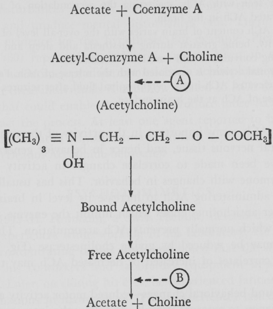
Fig. 5. Metabolism of acetylcholine. Choline acetylase, required for the synthesis of acetylcholine, acts at A. Cholinesterase, concerned with the destruction of acetylcholine, acts at B.
