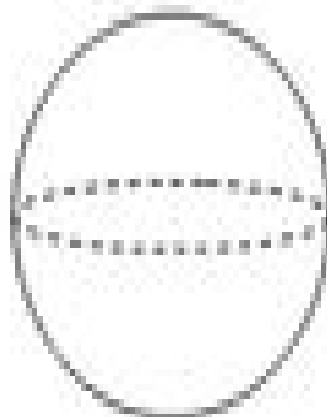
Sphere
