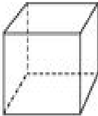
Cube
