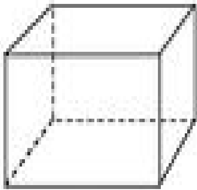
Rectangular solid
