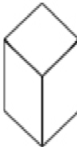
Cube
