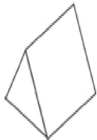
Triangular prism
