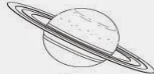
Saturn
