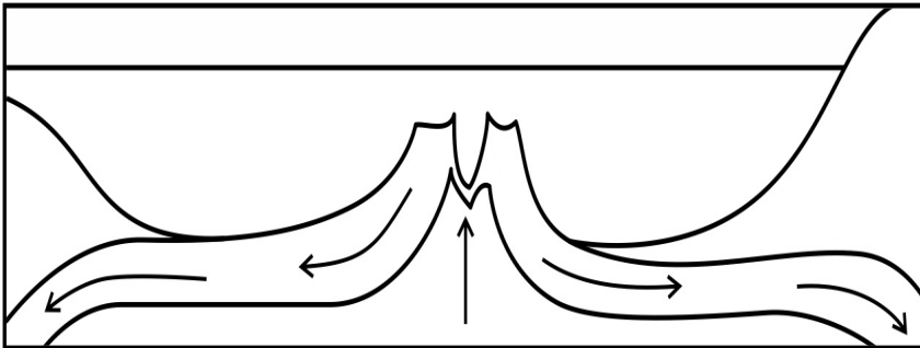
Advanced Rifting
