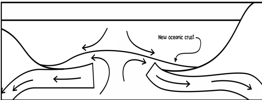
Seafloor Spreading
