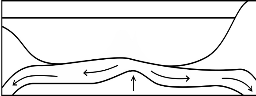
Early Rifting
