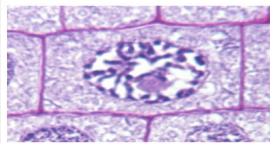
PROPHASE
