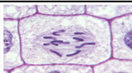
ANAPHASE
