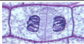
TELOPHASE
