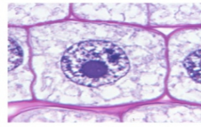
INTERPHASE
