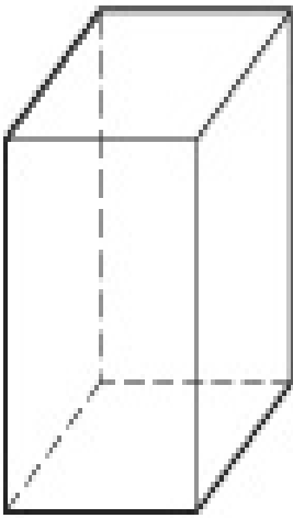
Rectangular solid
