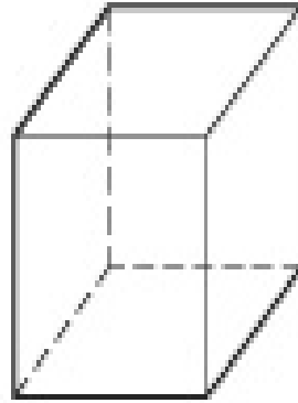
Cube
