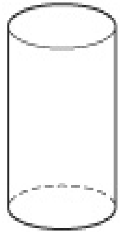
Cylinder
