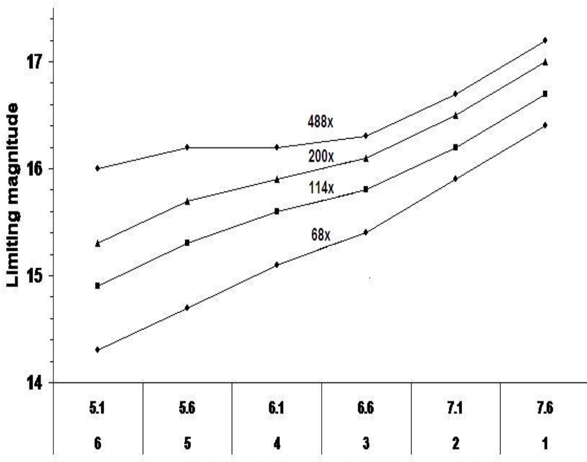
Bortle Scale 6-1 and zenith limiting magnitude
