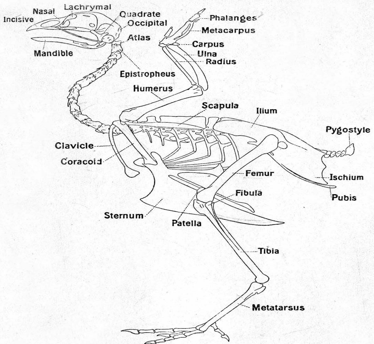
FIG. 1.—The Skeleton of the Fowl.
