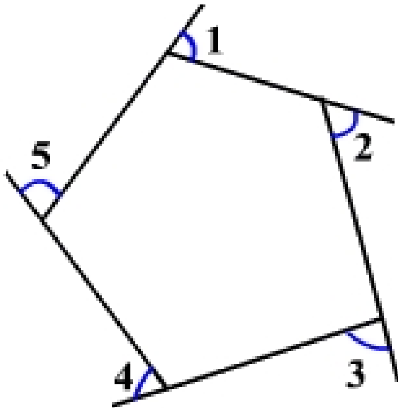
fig.:A 5-sided Polygon & exterior angles
