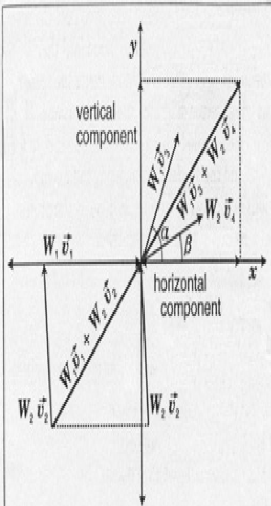
Fig. 1. Horizontal and vertical components of the linear-momentum equation
