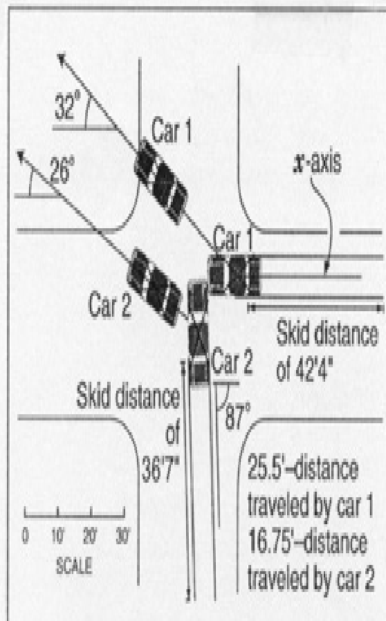
Fig. 2. Scale drawing showing the position of the cars at impact and the final resting positions after the accident
